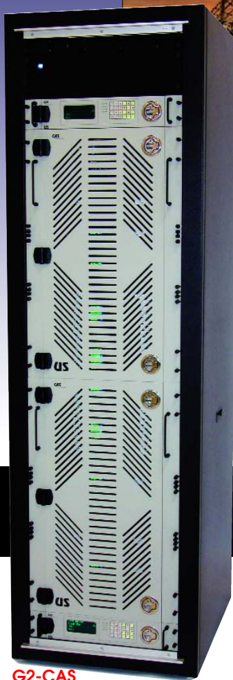
G2-CAS 12x128 and 128x12 Dual L-Band Matrix (Rx & Tx)
